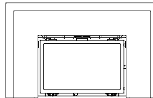
OVERSIZED SQUARE SURROUND
